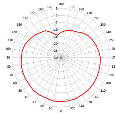
5.0G Vertical
