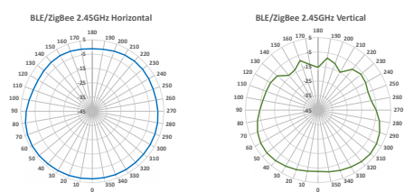
FAP-433G BLE/ZigBee antenna plots
