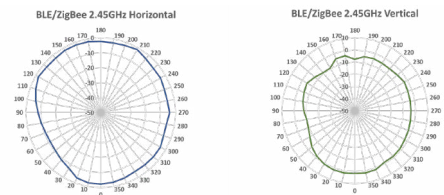
FAP-233G BLE/ZigBee antenna plots
