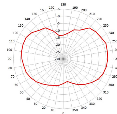
5.0G Vertical
