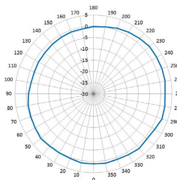
5.0G Horizontal
